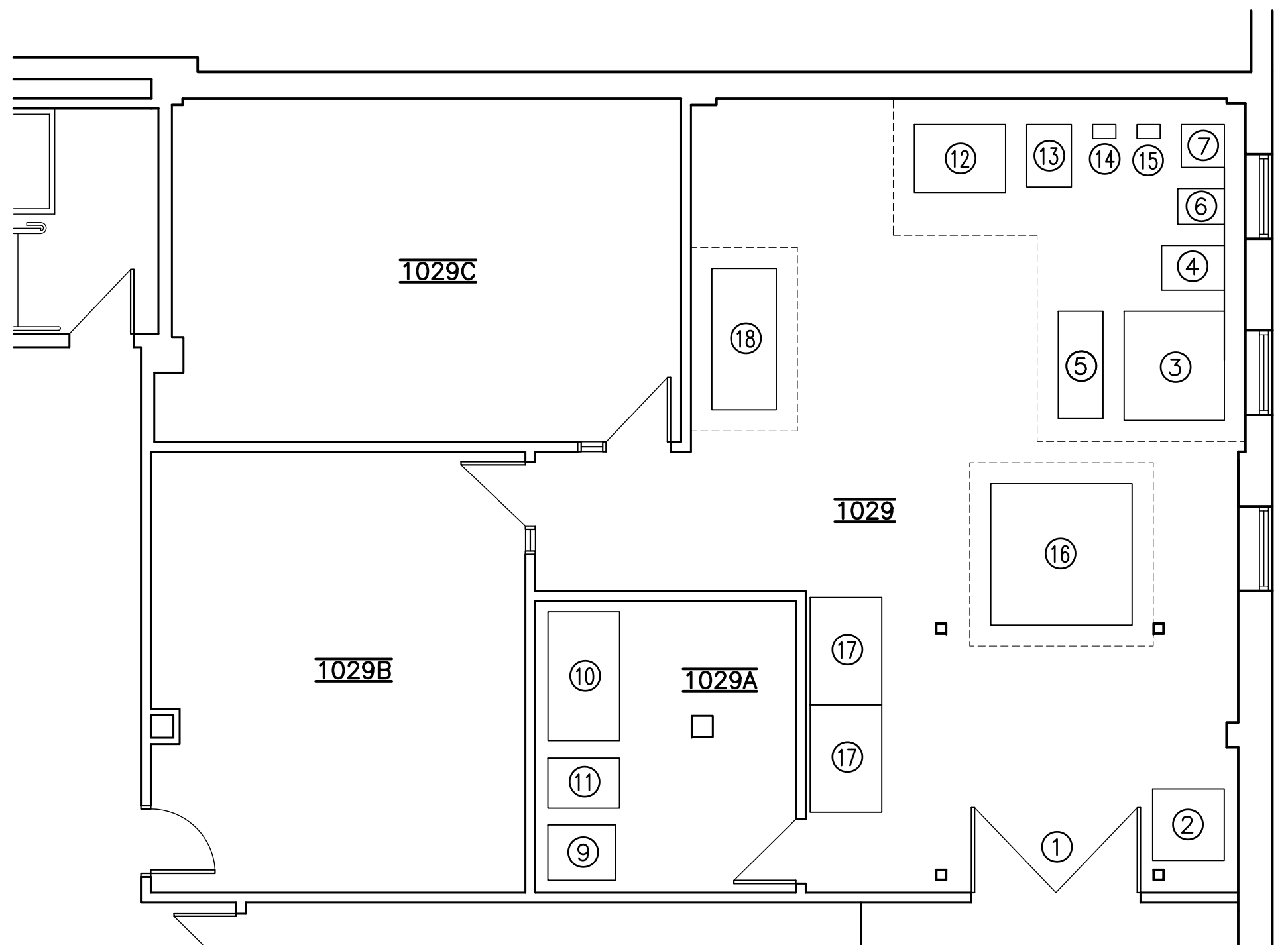
PROPOSED FLOOR PLAN SCALE: 1:75
